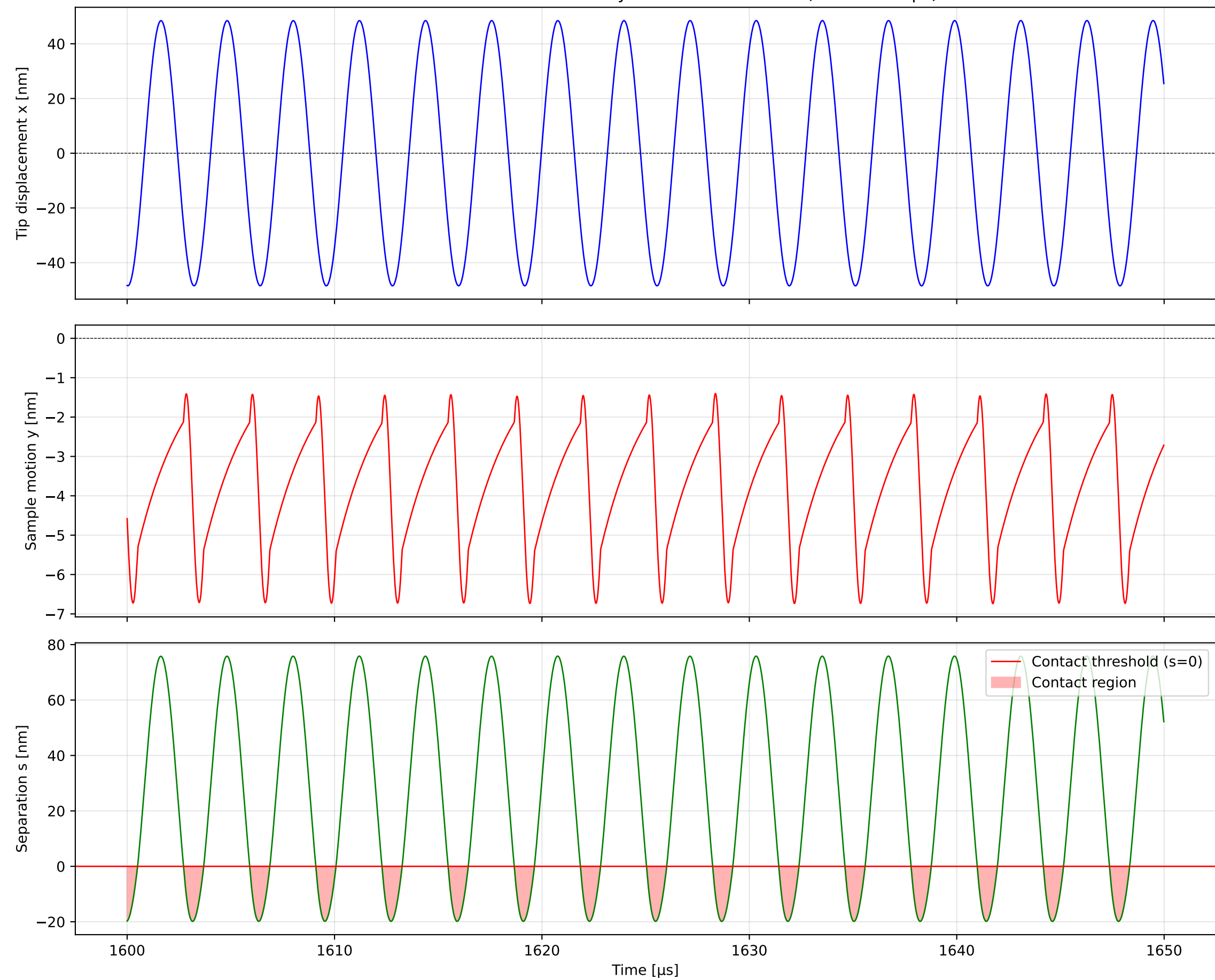
AFM DMT-KV Simulation: Steady-State Zoomed View (1600-1650 \mu\text{s} )
